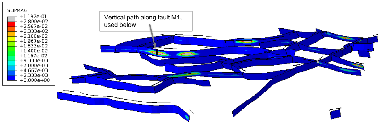
Figure 11.25 Contour plot of slip magnitudes in 2059 along faults of sub-model-1 for the base case production scenario
