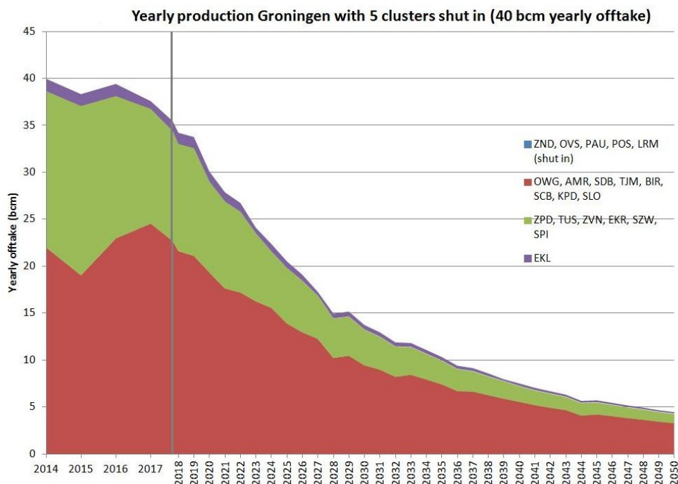
Figure 3.3b Production forecast using the G2 model with the 5 northern clusters closed-in with production curtailment to 40 Bcm/year (as the field is not able to produce at higher levels, this is also the market demand scenario). The stacked contributions to the gas production of the northern clusters (blue; not shown), the central clusters (red), the southern clusters (green) and Eemskanaal cluster (purple) is shown. The time-axis has been split to highlight the period 2014 to 2017.
