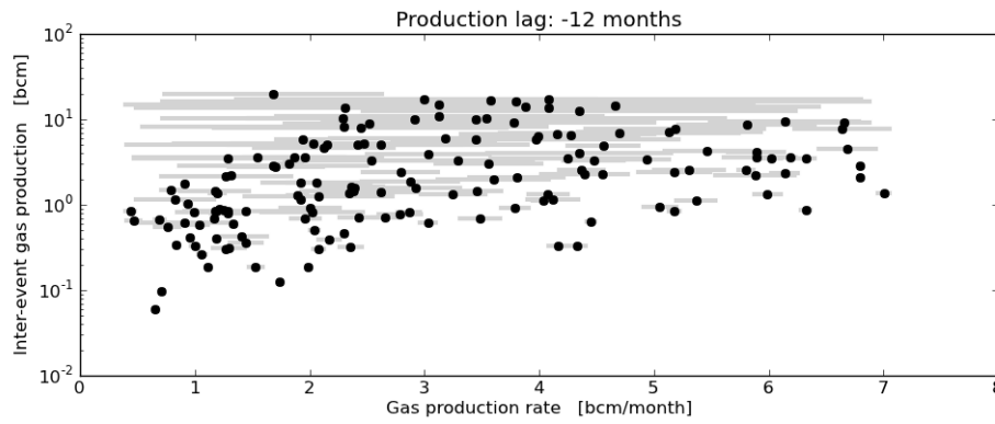
Figure 6.7 Inter-event gas production exhibits little sensitivity to the rate of gas production. To avoid any bias of event clustering, all events within 3 days of the previous event were excluded. Dots and grey bars denote the average and the range of inter-event production rates respectively; in some instances the grey bar is so small as to be covered by the black dot; (a) and (b) represent 0- and 12-months lag times, respectively.
