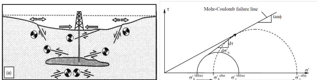
Figure 9.5 Principle of seismicity occurring outside the reservoir (left, taken from Segall, 1989) and depletion-induced seismicity (right, taken from Mulders, 2003)
