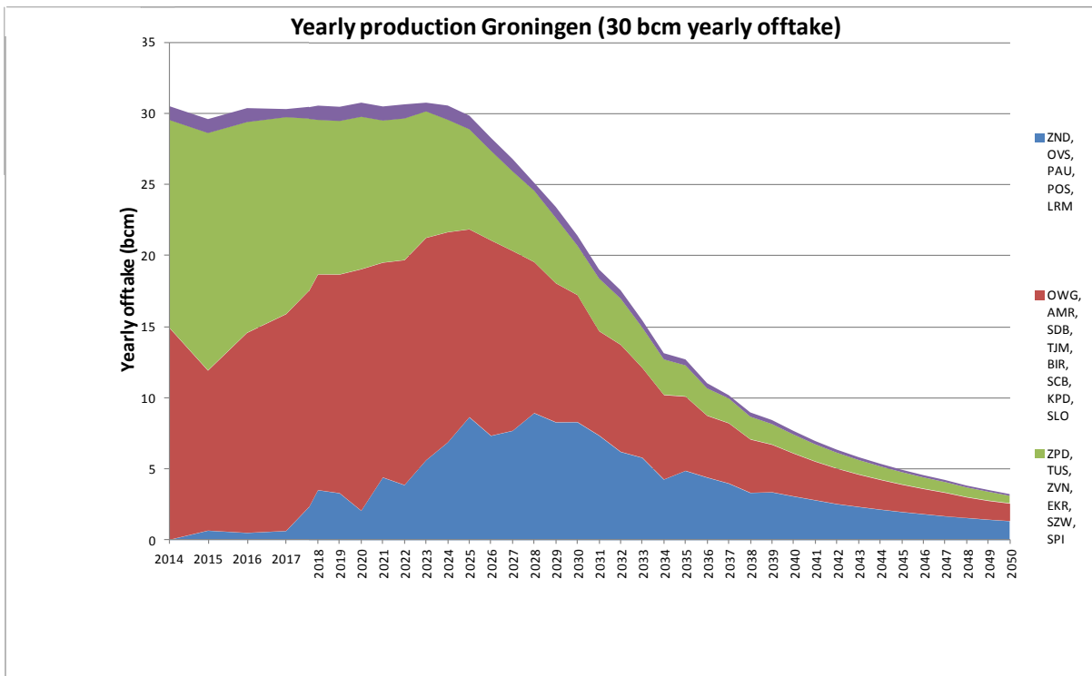
Figure 3.1b Production forecast using the G1 model for the alternative production philosophy with production curtailment to 30 Bcm/year. The stacked contributions to the gas production of the northern clusters (blue), the central clusters (red), the southern clusters (green) and Eemskanaal cluster (purple) is shown. The time-axis has been split to highlight the period 2014 to 2017.
