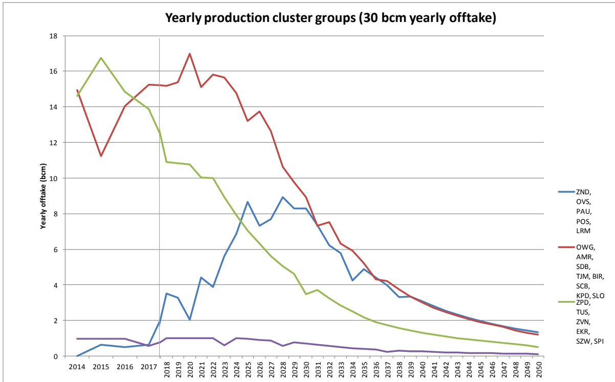
Figure 3.1a Production forecast using the G1 model for the alternative production philosophy with production curtailment to 30 Bcm/year. The contributions to the gas production of the northern clusters (blue), the central clusters (red), the southern clusters (green) and Eemskanaal cluster (purple) is shown. The time-axis has been split to highlight the period 2014 to 2017.
