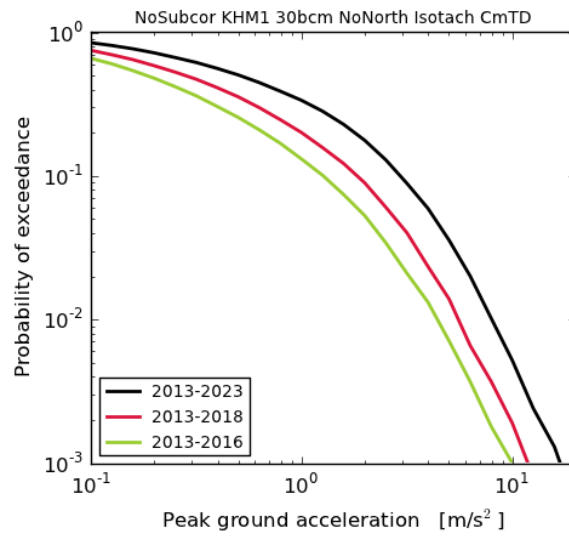
Figure 5.8 The probability of exceedance for the maximum peak ground acceleration within the Groningen Field for three different assessment intervals: 3, 5, and 10 years.
