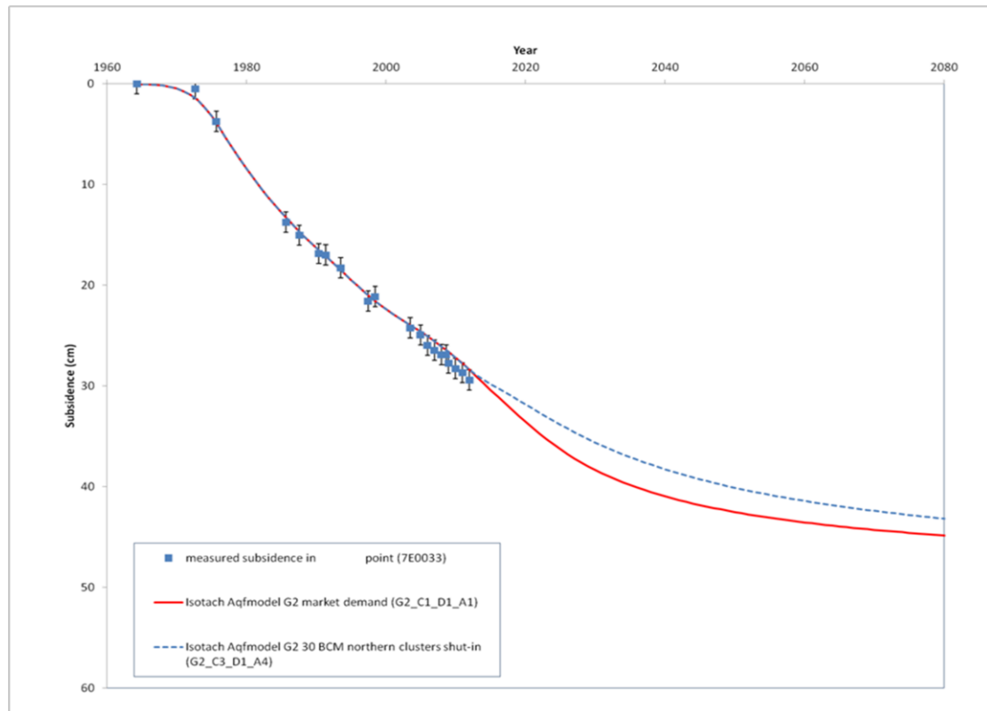
Figure B.1 Comparison of subsidence forecast at the location of benchmark 7E0033 according to the two different production scenarios. For ease of comparison with figure 4.30 in the “Technical Addendum to the Winningsplan Groningen 2013” the same benchmark location was chosen.
