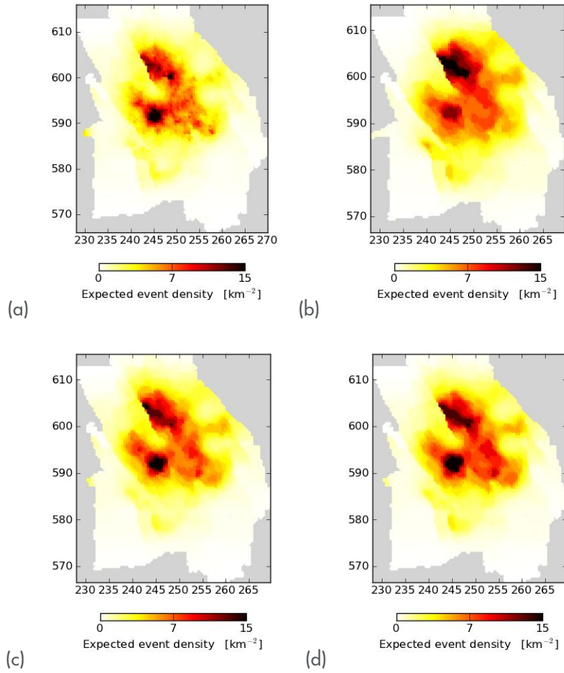
Figure 8.14 Event density maps for the interval 2013 to 2023 based on four different models of reservoir compaction: (a) linear, (b) bi-linear, (c) time-decay, and (d) Isotach. The horizontal and vertical scales are Rijkzdriehoek (RD) coordinates in km.
